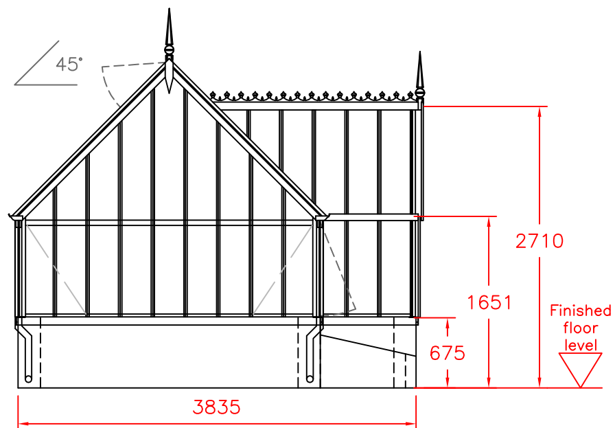
GABLE ELEVATION
