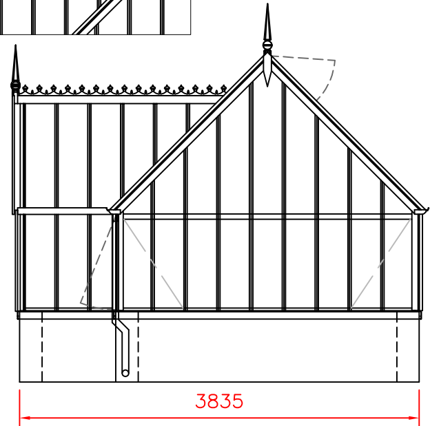
GABLE ELEVATION
