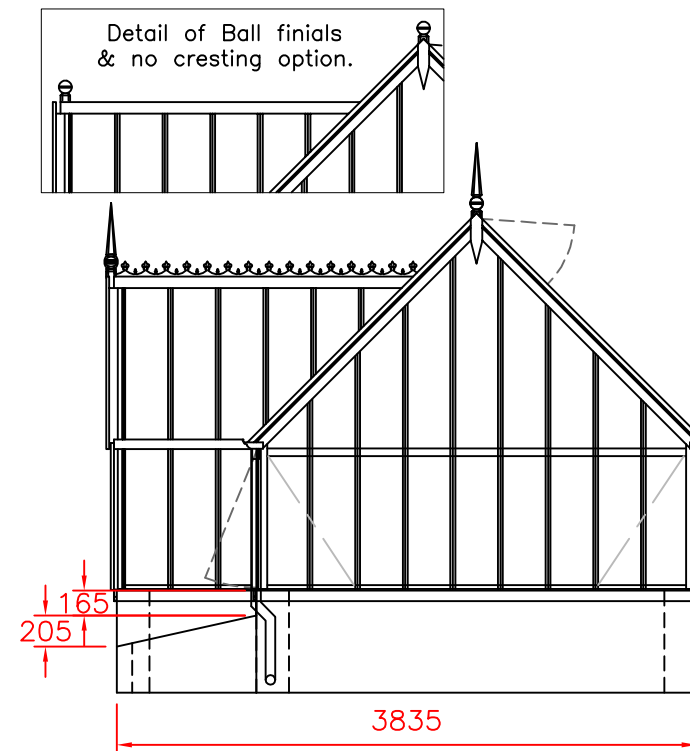
GABLE ELEVATION
